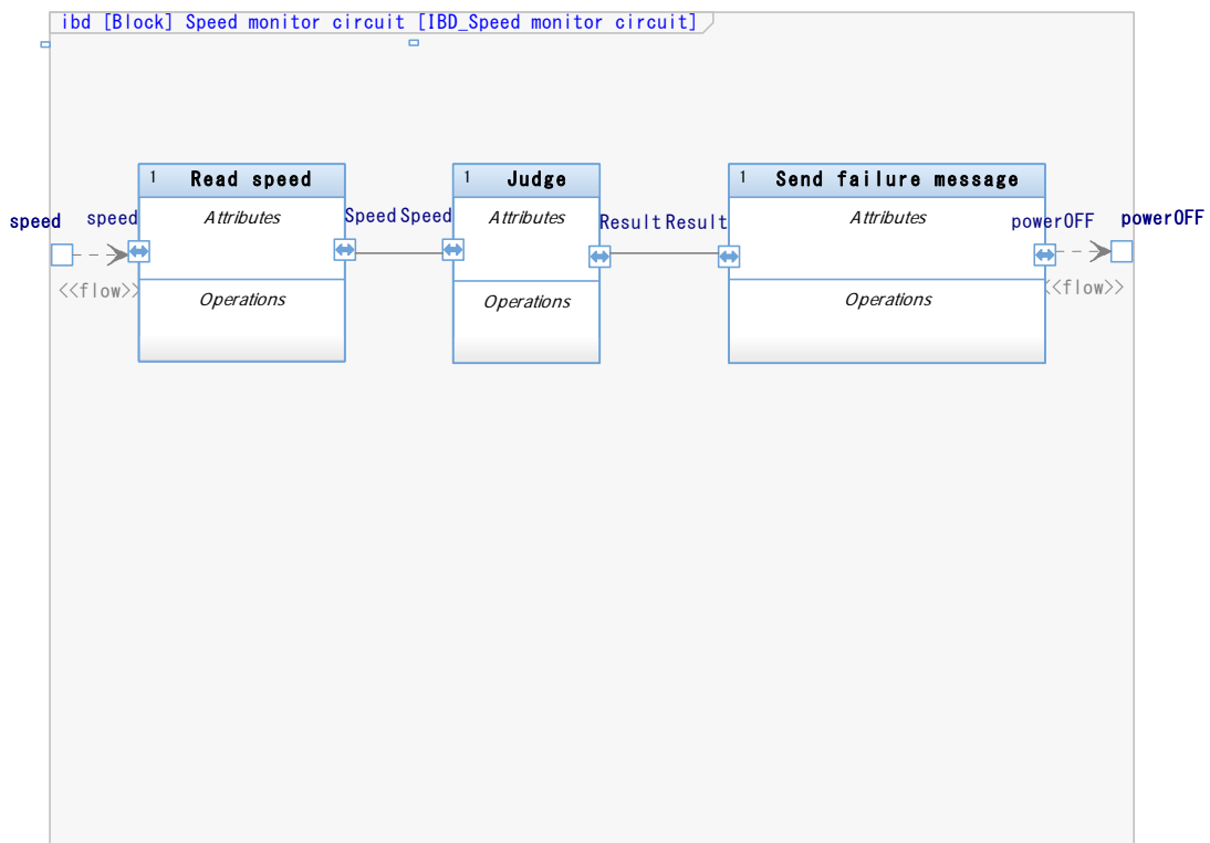
Figure 3-6 Internal block diagram (Original diagram is in Japanese)
