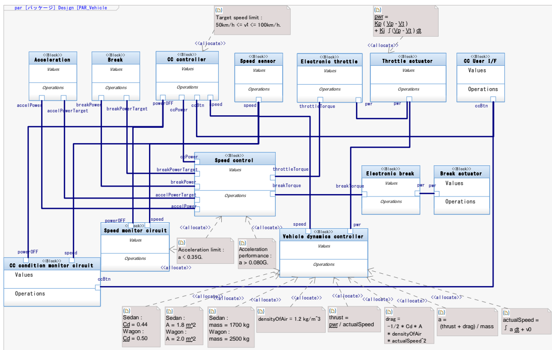
Figure 3-5 Parametric diagram (Original diagram is in Japanese)
