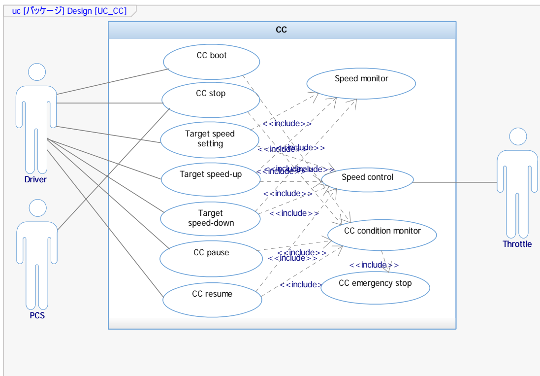
Figure 3-2 Use case diagram (Original diagram is in Japanese)
