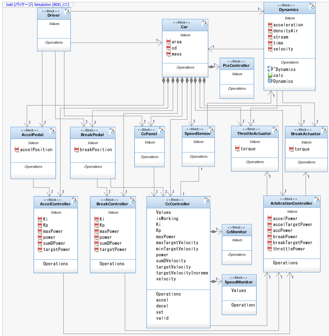
Figure 3-7 Block definition diagram (Implementation)
